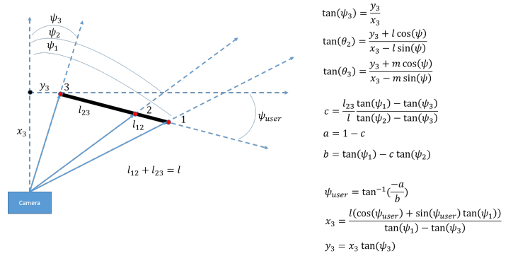
Fig. 5: State Reconstruction. By obtaining angular position measurements of three LEDs with known offsets, it is possible to fully reconstruct the state in a plane.
